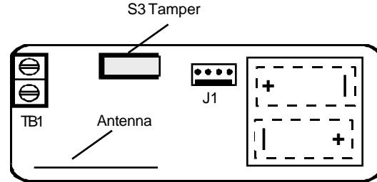
Figure 2 - PCB Layout
